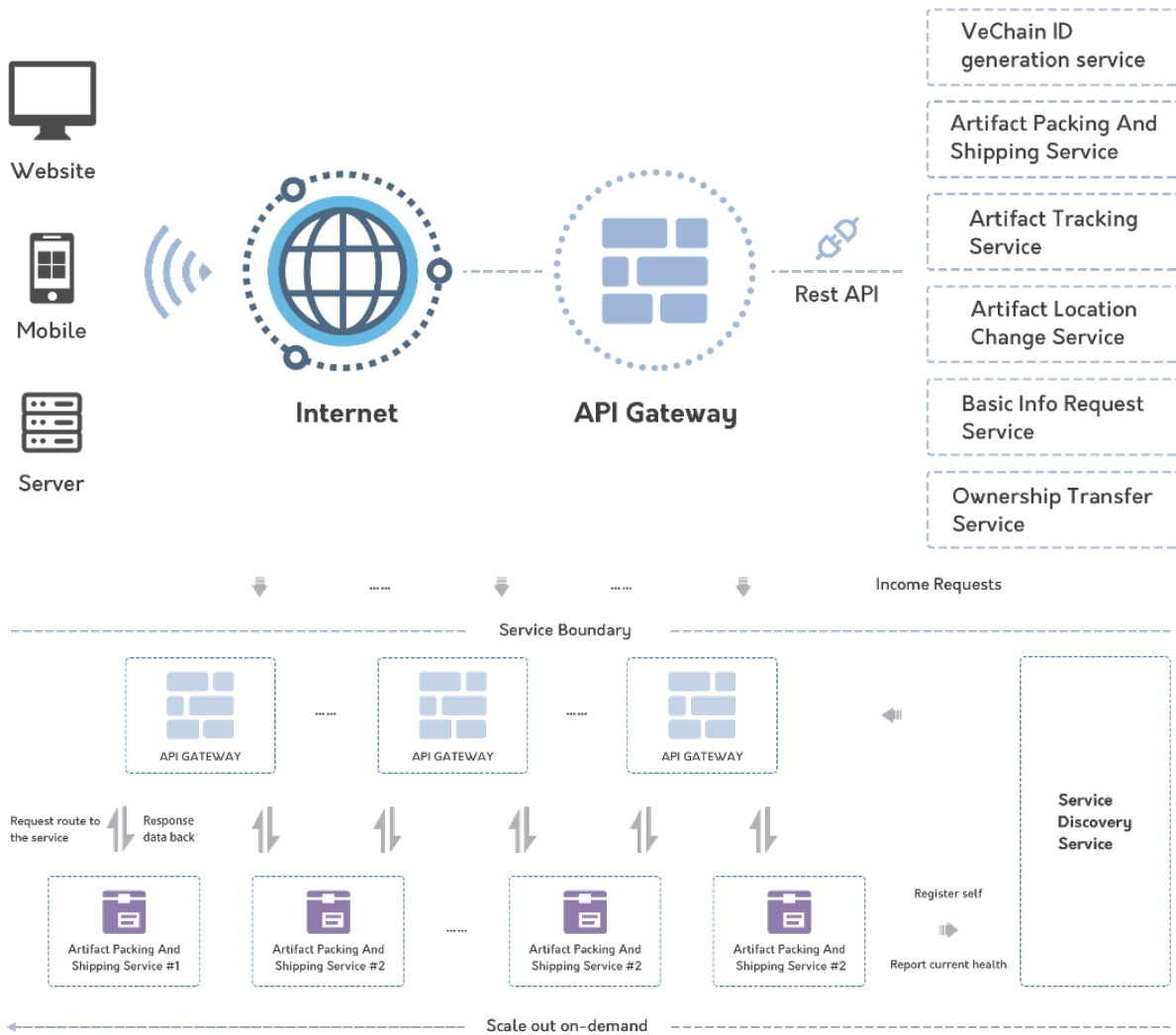
Figure 5.3.5.1 API Gateway-1
