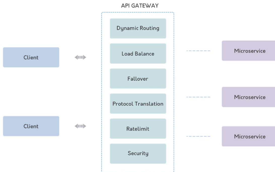
Figure 5.3.5.2 API Gateway
